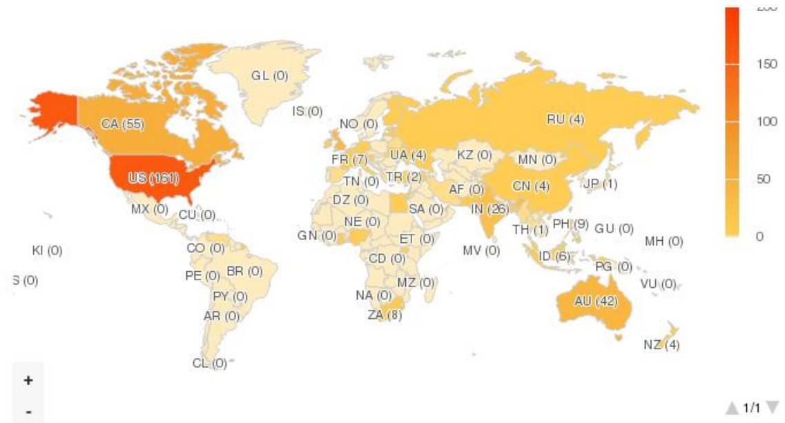
Heat Map
